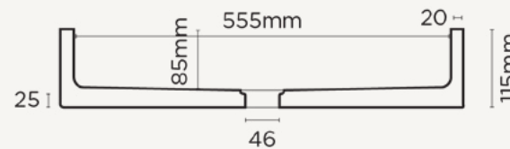
SECTION VIEW
