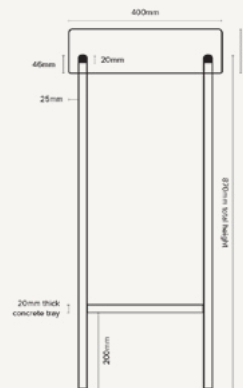
SECTION VIEW
