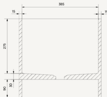
SECTION VIEW
