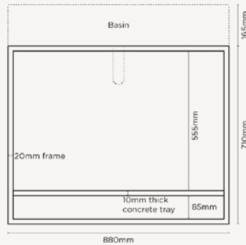
SECTION VIEW
