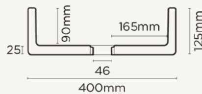
SECTION VIEW
