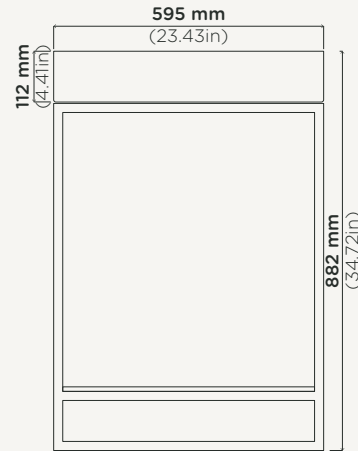
Elevation View
