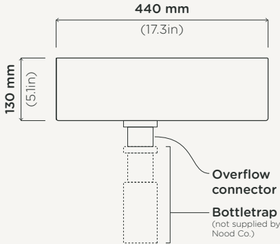
Elevation View
