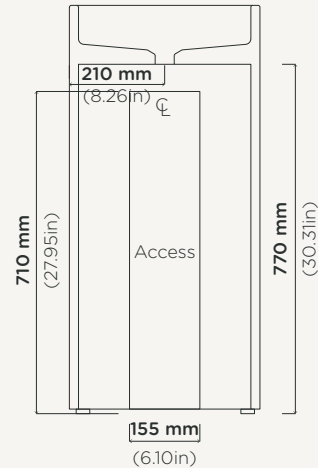
Section View
