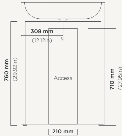
Section View
