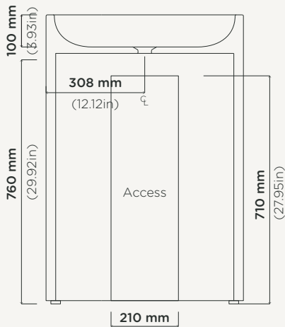
Section View
