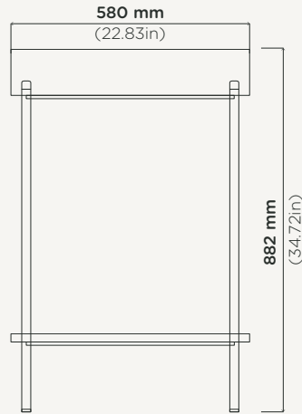
Elevation View
