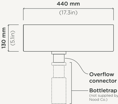
Elevation View
