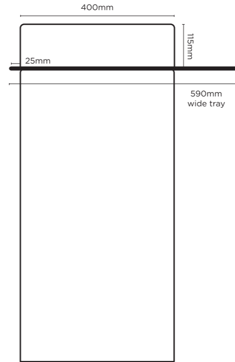
CYLINDER + 1 TRAY - RIGHT
